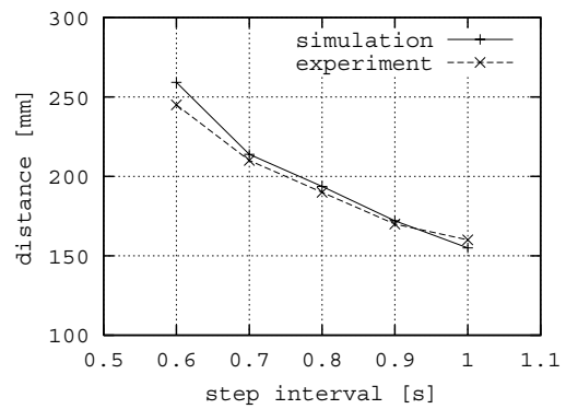
Fig. 13. Comparison between simulation and experimental results for voltage pattern BF
