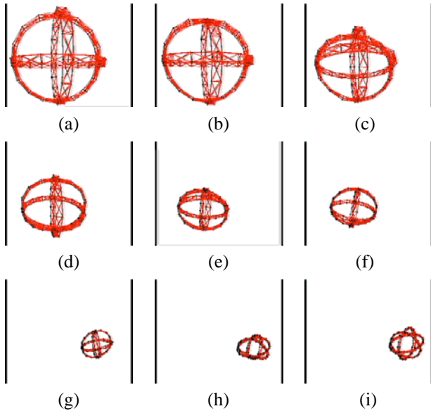
Fig. 9. Crawling of a spherical soft robot
