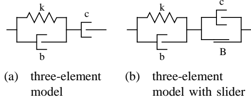
Fig. 4. Model of SMA coils
