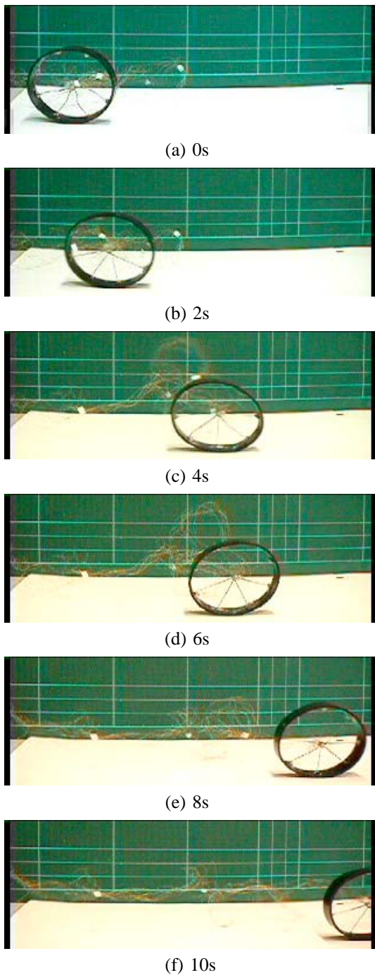
Fig. 12. Circular soft robot crawling
