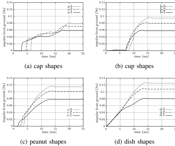
Fig. 16. Impulse from ground during jumping
